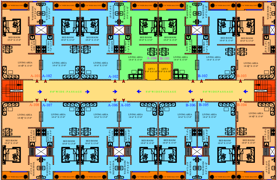
TYPICAL UNIT CLUSTER LAYOUT PLAN
